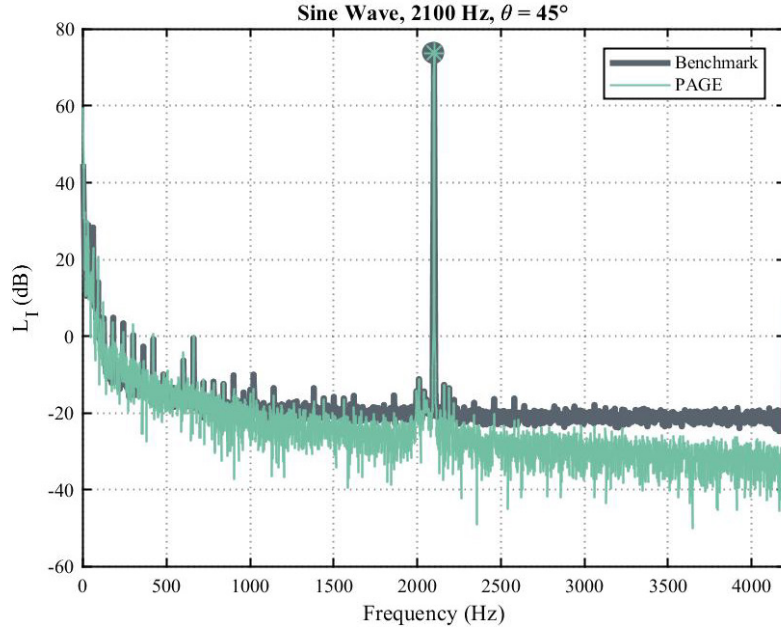
Figure 3.11: For a 2100 Hz sine wave in an anechoic chamber, a benchmark of I = \frac{p_{rms}^2}{\rho_0 c} is compared to the PAGE calculation of active intensity for a probe with a 45° angle of rotation. Markers on each curve are at the frequency of the sine wave.
