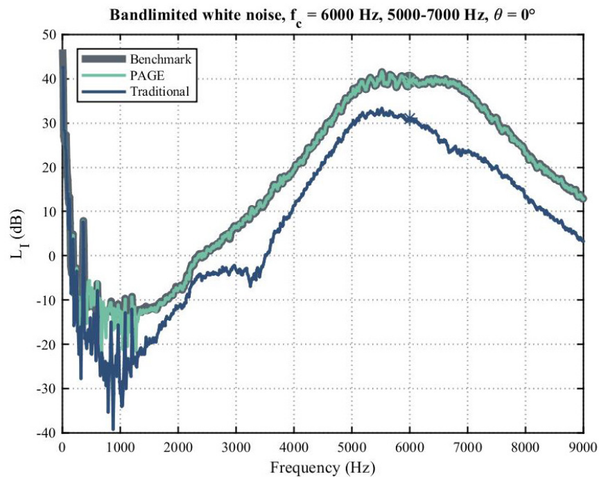
Figure 3.45: For filtered white noise from 5000-7000 Hz in an anechoic chamber, a benchmark of I = \frac{p_{rms}^2}{\rho_0 c} is compared to active intensity calculated using the PAGE method and the traditional method for a probe at a 0^\circ angle of rotation. A marker on each curve is at f_c .
