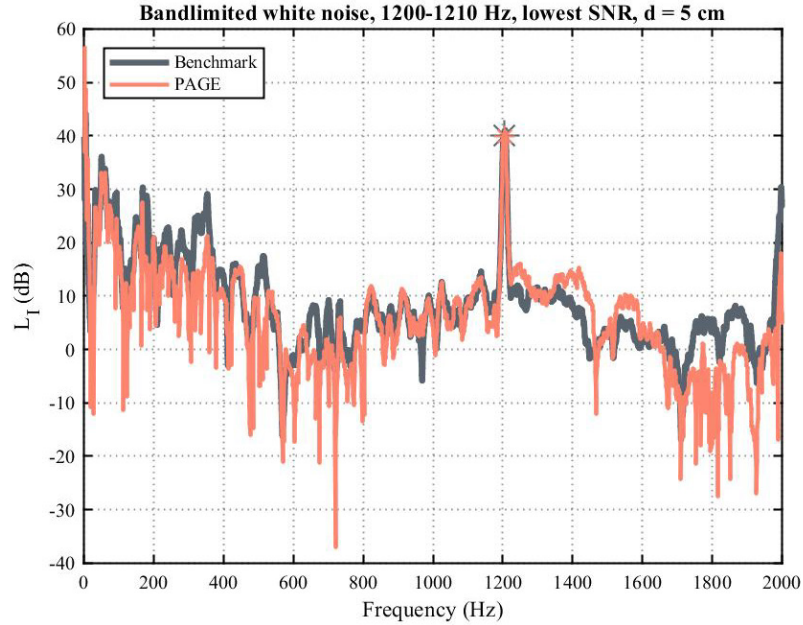
Figure 2.15: For filtered white noise from 1200-1210 Hz in the plane wave tube and additive noise resulting in the lowest tested SNR, a benchmark of I = \frac{p_{rms}^2}{\rho_0 c} is compared to active intensity calculated using the PAGE method. A marker on each curve is at the center of the bandwidth, in this case at 1205 Hz.
