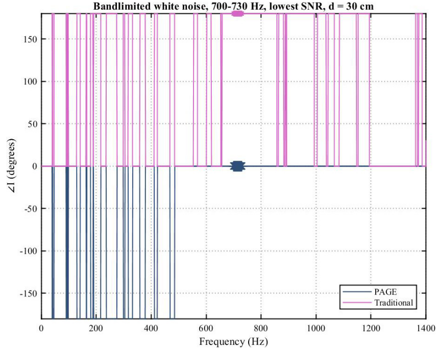
Figure 2.28: For filtered white noise from 700-730 Hz in the plane wave tube and additive noise resulting in the lowest tested SNR, intensity direction calculated using the PAGE method is compared to intensity direction calculated using the traditional method. Markers on each curve are at each frequency of the bandwidth, in this case from 700-730 Hz.
