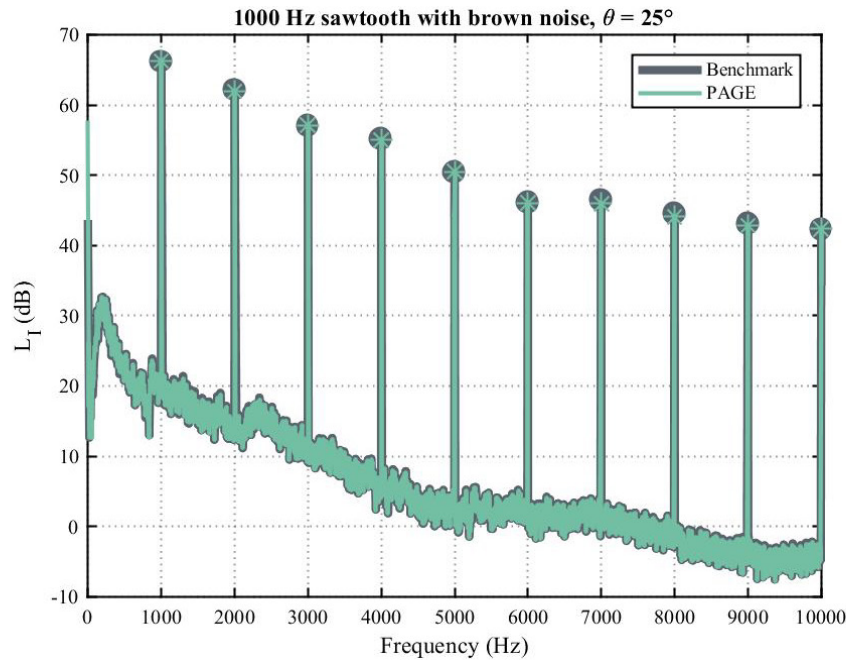
Figure 4.6: For a speaker broadcasting a 1000 Hz sawtooth wave ( \theta_s = 0^\circ ) and another speaker broadcasting brown noise (noise case 1, \theta_n = 25^\circ ), a benchmark of I = \frac{v_{rms}^2}{\rho_0 c} is compared to active intensity calculated using the PAGE method. Markers on each curve are at the frequencies of the sawtooth wave.
